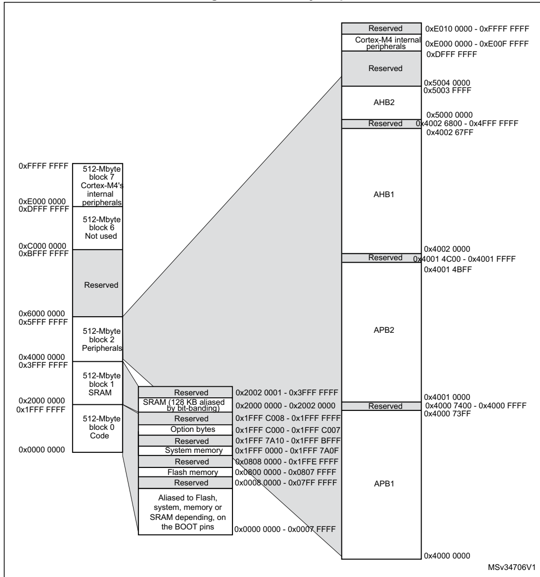
Figure 14. Memory map
