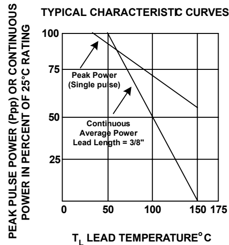
FIGURE 1 DERATING CURVE
