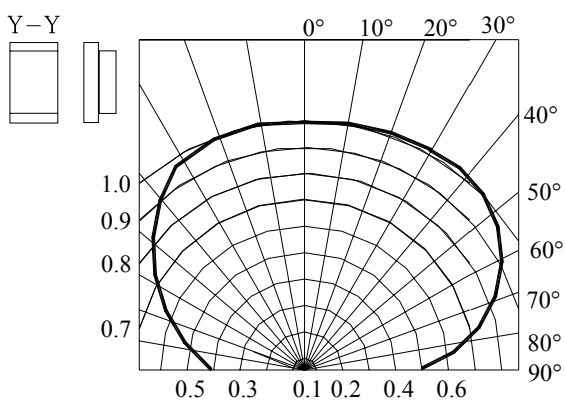
Fig.6 Relative Intensity vs. Angle
