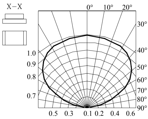
Fig.5 Relative Intensity vs. Angle
