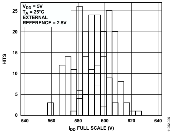
Figure 24. I_{DD} Histogram with External Reference
