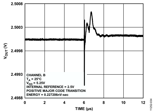
Figure 33. Digital-to-Analog Glitch Impulse
