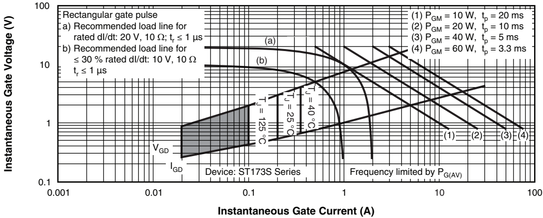
Fig. 15 - Gate Characteristics
