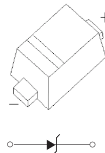
SOD-723
