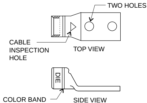
WP91412 Connector (Straight)
