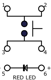
▲ CIRCUIT: SPST
