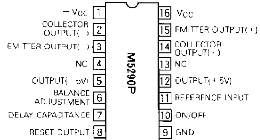
Outline 16P4
