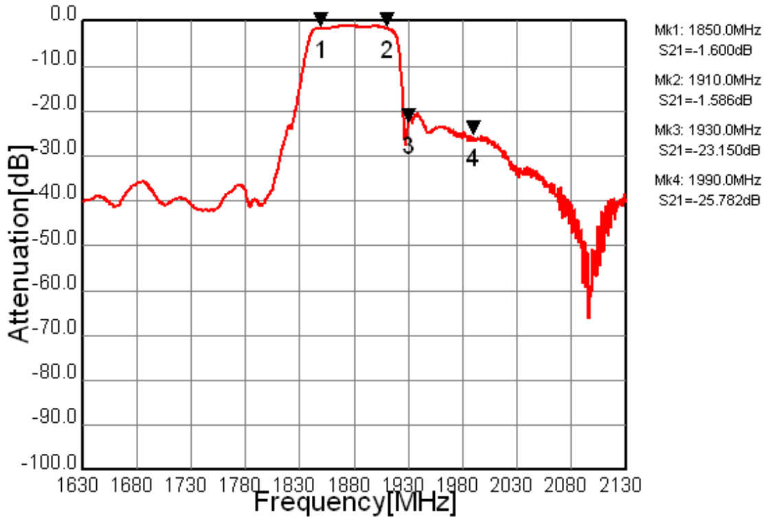
Fig.1 Pass-band Characteristics
