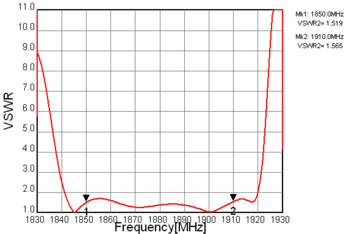
Fig.5 Output VSWR
