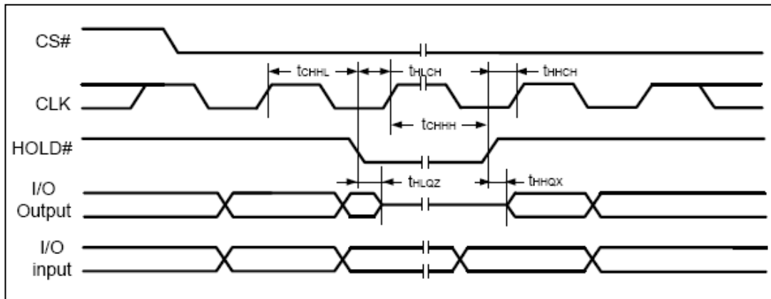
Figure 28 Hold timing
