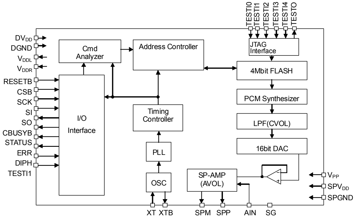
Block Diagram of ML22Q553-NNN/ML22Q553-xxx
