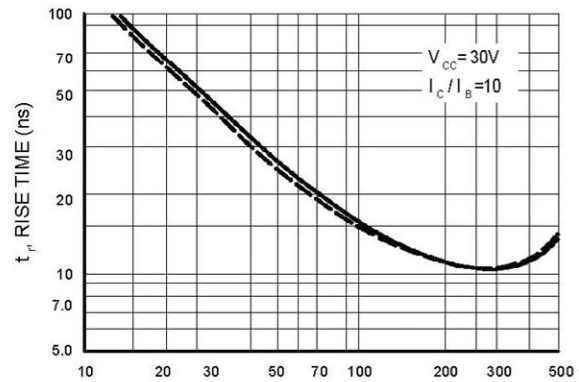
Figure 6. Rise Time
