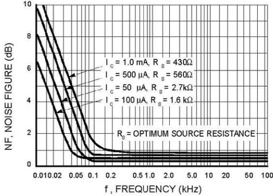
Figure 8. Frequency Effects
