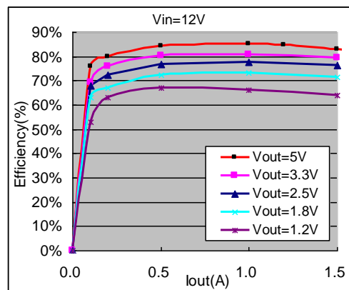
Efficiency ( V_{IN}=12V )
