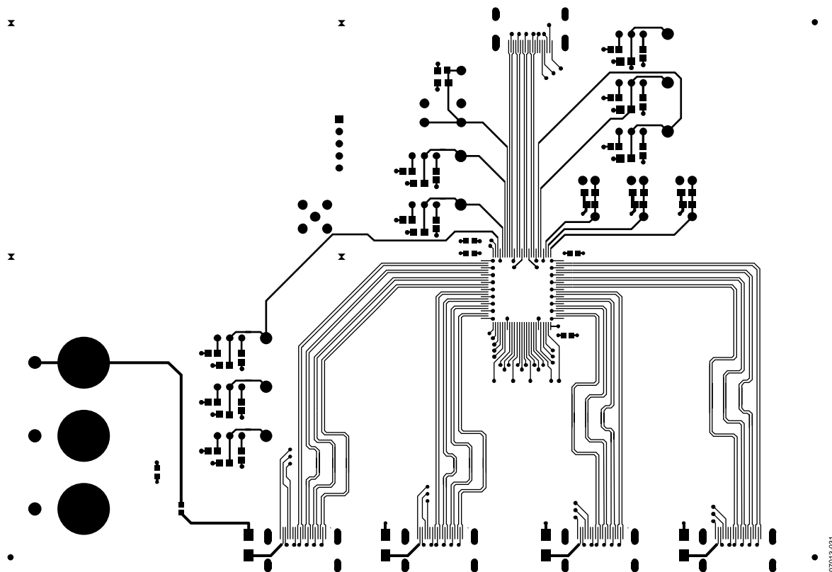
Figure 31. Layout of the TMDS Traces on the AD8191A Evaluation Board (Only Top Signal Routing Layer is Shown)
