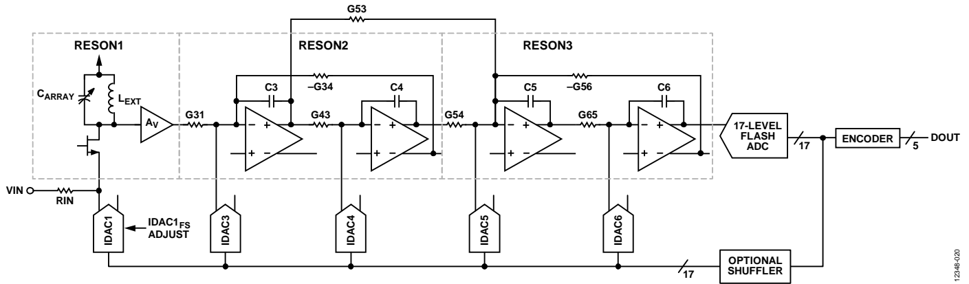
Figure 68. Simplified Single-Ended Representation of the Band-Pass Σ-Δ ADC Modulator
