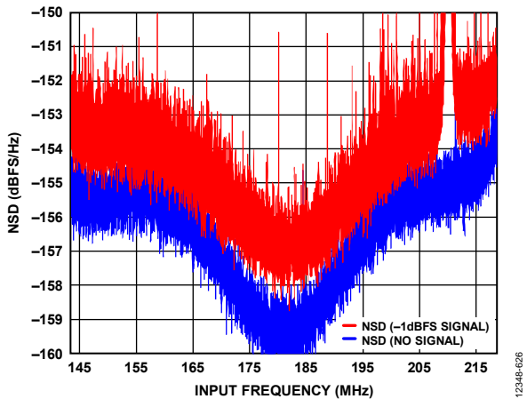
Figure 23. NSD With and Without Full-Scale CW at 210 MHz
