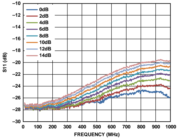
Figure 94. Differential S11 vs. Frequency for Different Attenuator Settings
