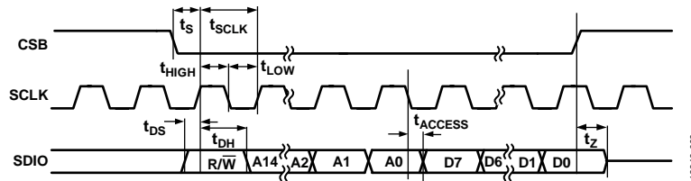
Figure 147. SPI 3-Wire Read Operation Timing
