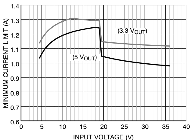
Figure 28. NCV890101 Load Current Capability with 4.7 \mu\text{H} Inductor
