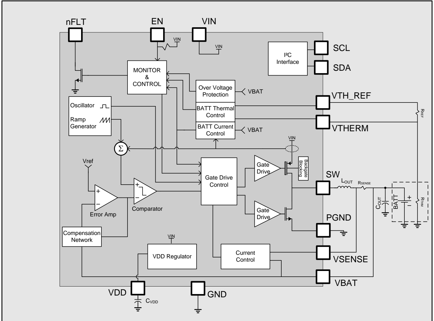
Figure 2: TS55001 Block Diagram
