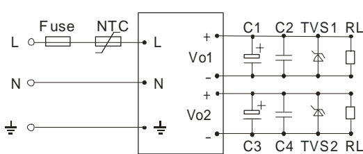
LH**-10D**E(Isolate Twin Output) (figure 2)
