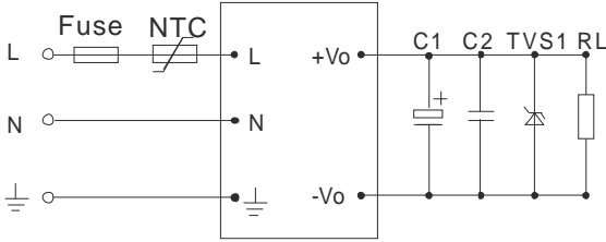
LH**-10B**E( Single Output) (figure 1)
