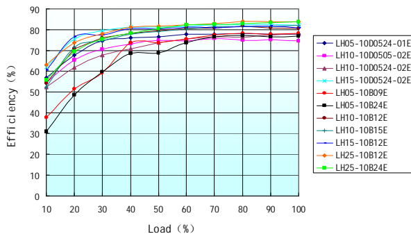
Load VS Efficiency curve (Vi=220Vac)
