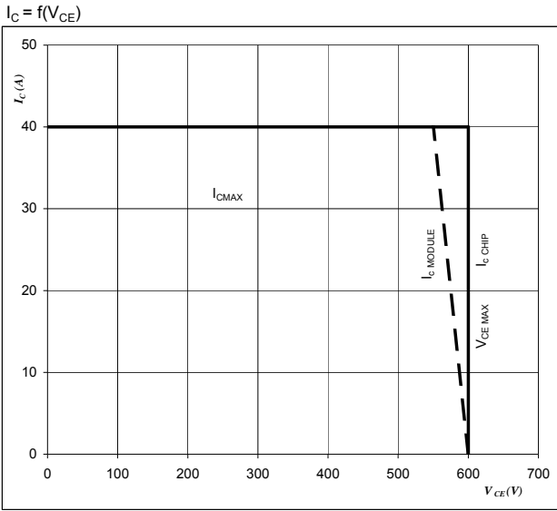
Figure 29 IGBT
