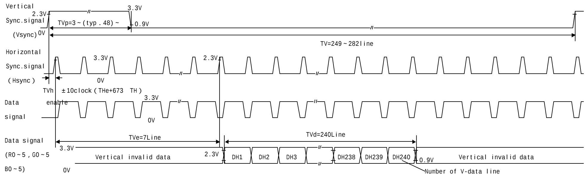
Fig.7-1 Input signal waveforms (EMAP:active)
