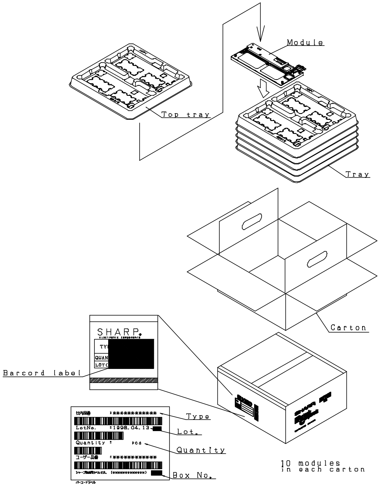
Fig.3 Packing Form
