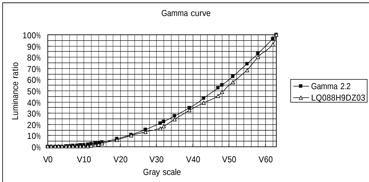
Gamma curve & gamma ratio (Ta=25 ) [Reference value]
