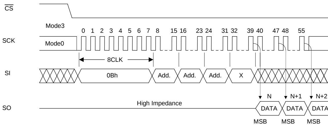
Figure 5-b 5 Bus Read
