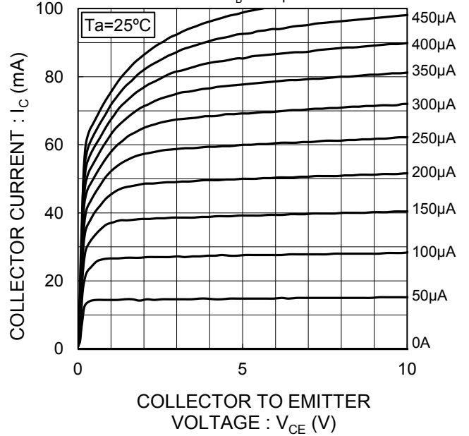
Fig.2 Grounded emitter output characteristics I_B = 500\mu A
