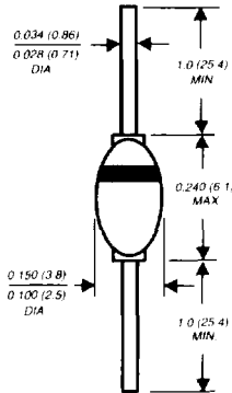
DO-204AP
