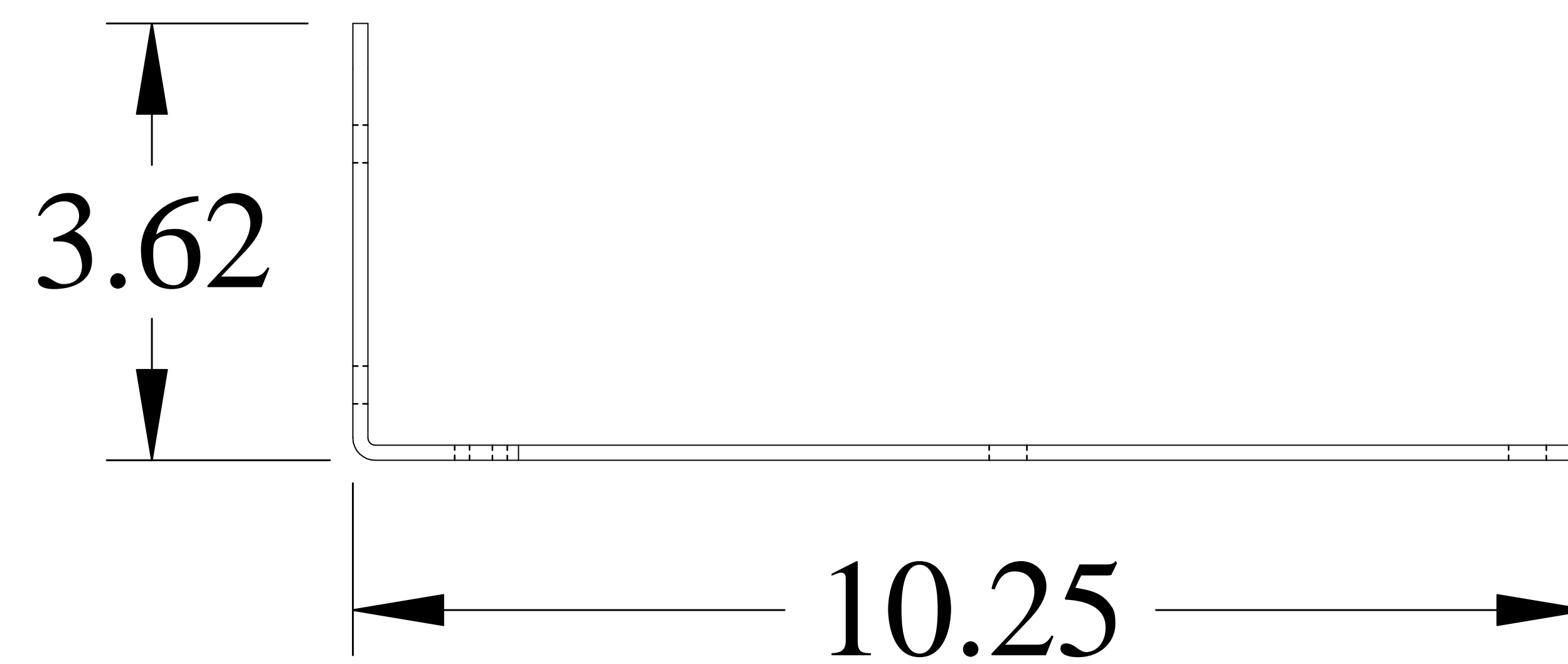
TOP VIEW
