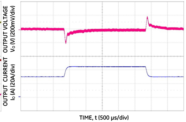
Figure 4. Typical Transient Response to 1A/µs Step Change in Load from 50% to 75% to 50% of Full Load, C_o=2400\mu F and 48 V dc Input.
