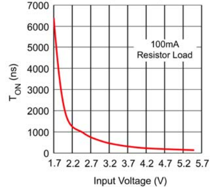
T_{ON} Delay vs. Input Voltage
