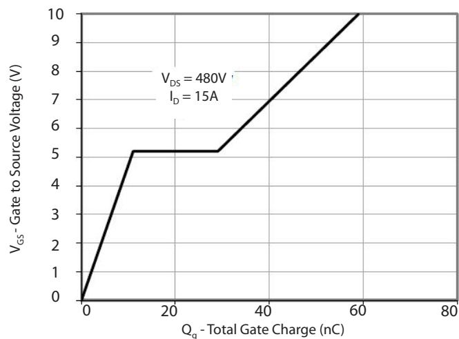
Gate Charge
