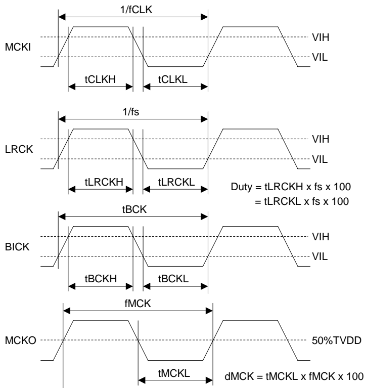
Figure 3. Clock Timing (PLL Slave mode)
