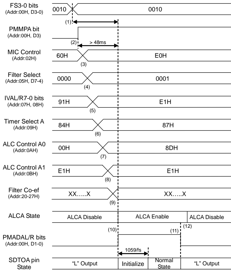
Figure 57. Microphone Input Recording Sequence (LIN1/RIN1 → ADCA → ALCA → Audio I/F → SDTOA)
