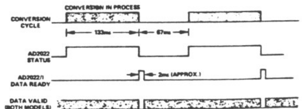
Figure 8. AD2022 Timing Diagram
