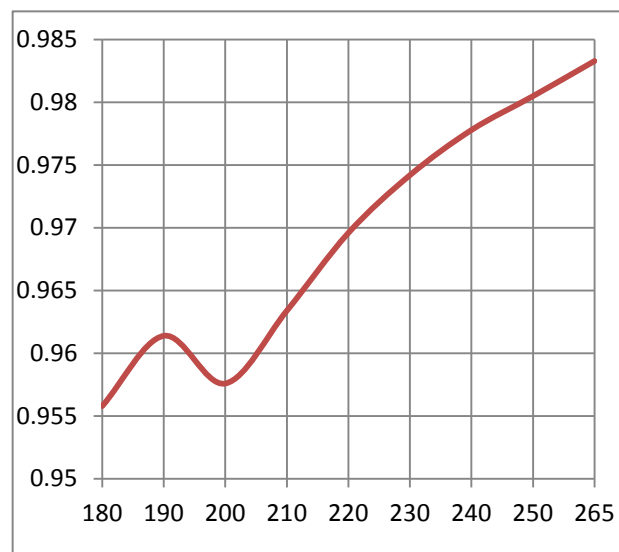
PF Value vs. AC Input Voltage (V)
