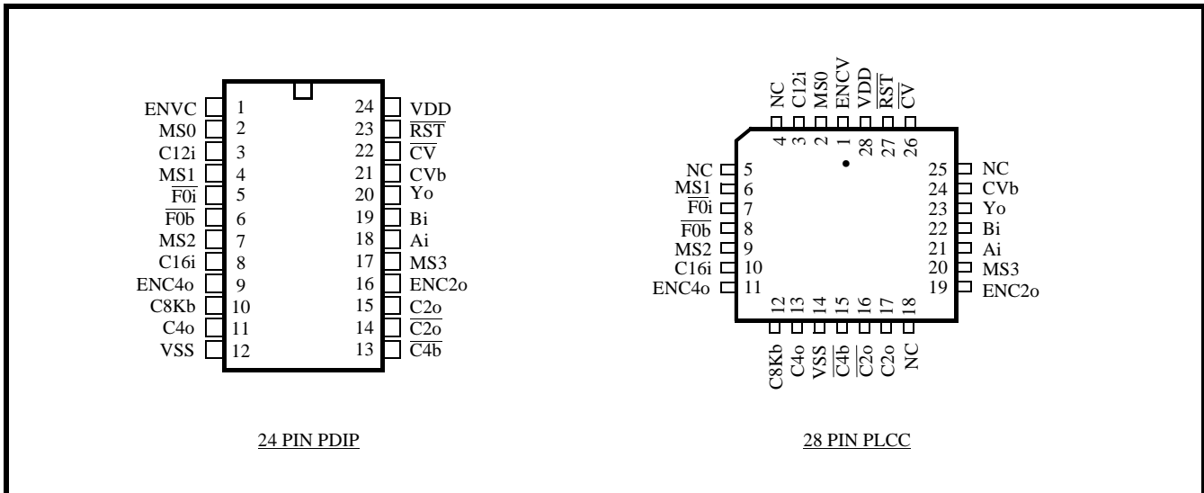
Figure 2 - Pin Connections
