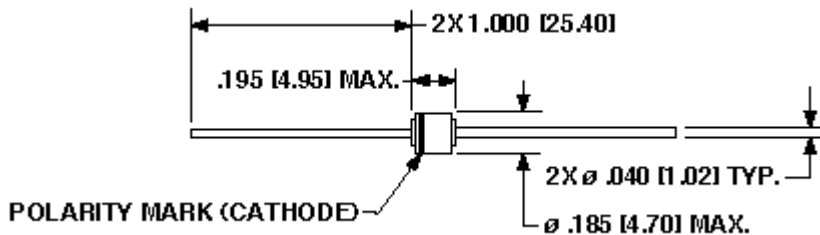
PACKAGE G for 1N6138 thru 1N6173A (1500 W)
