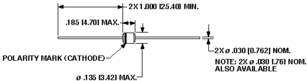
PACKAGE E for 1N6102 thru 1N6137A (500 W)
