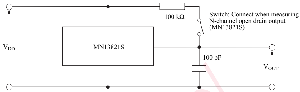
Figure 3. Circuit for Measuring the Output Characteristics
