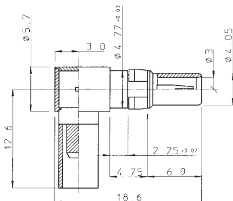
socket contact
