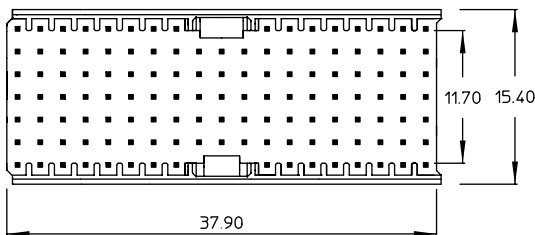
Standard loading patterns (seen from mating side)
