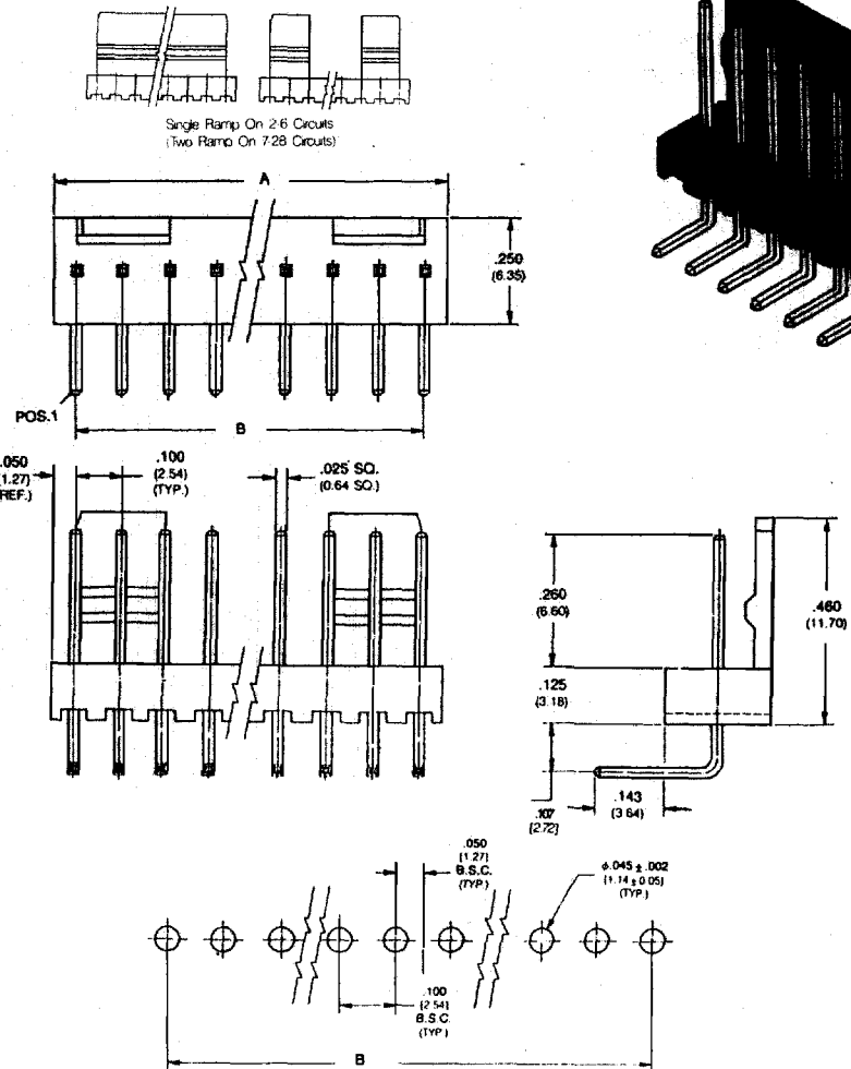
RECOMMENDED P.C. BOARD PATTERN
