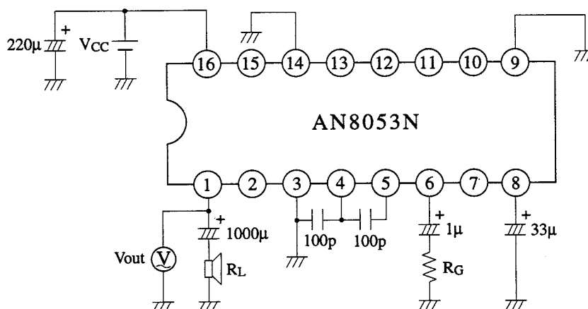
Test Circuit 8
