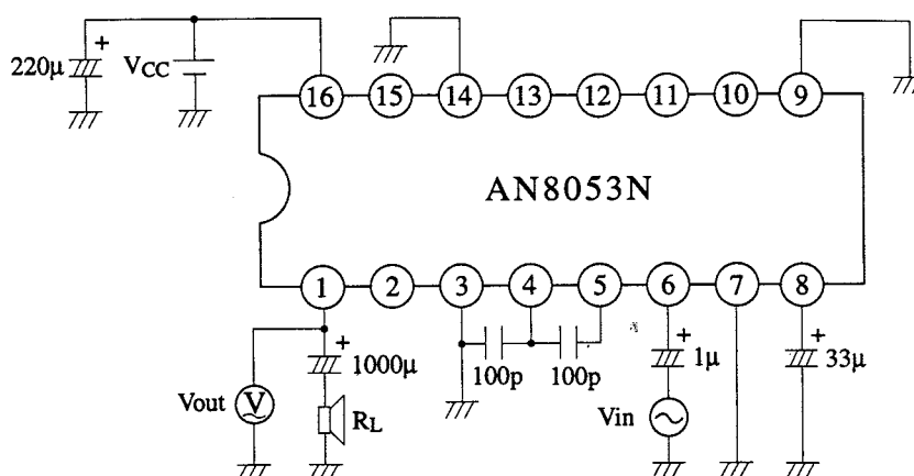
Test Circuit 8
