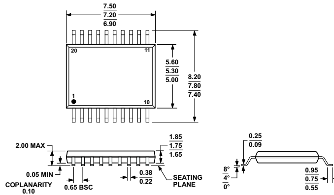
Figure 33. 20-Lead Shrink Small Outline Package [SSOP] (RS-20)
