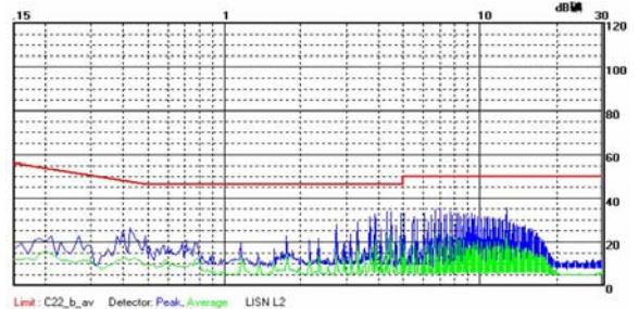
WRA2415P-3WR2 CE(Class B, Negative line)
