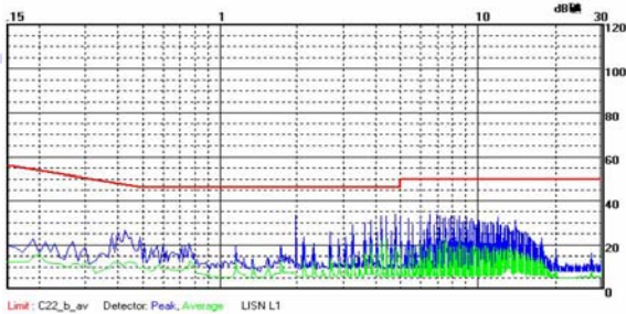
WRA2415P-3WR2 CE(Class B, Positive line)
