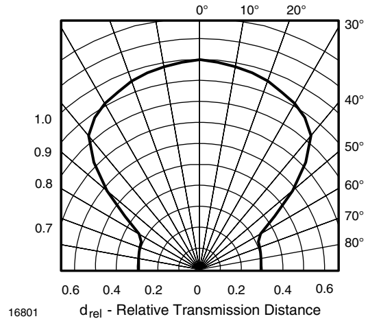
Fig. 12 - Horizontal Directivity
