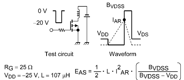
Fig. 8.15 Test Circuit/Waveform
