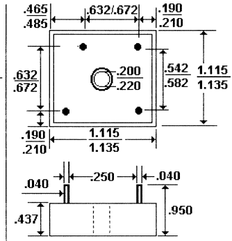
Metal Case/Wire Leads
