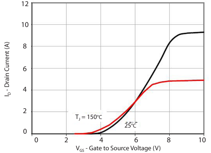
Transfer Characteristics
