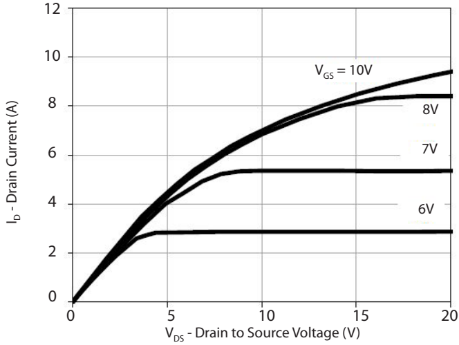
Output Characteristics
