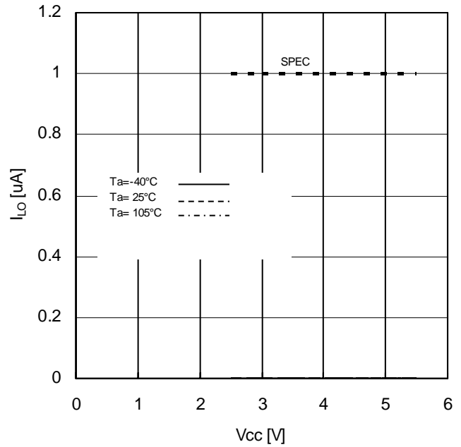
Figure 10. Output Leak Current vs Supply Voltage
