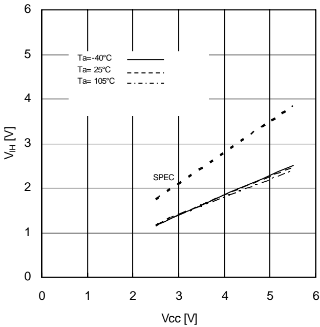
Figure 5. "H" Input Voltage vs Supply Voltage (CSB,SCK,SI,HOLDB,WPB)
