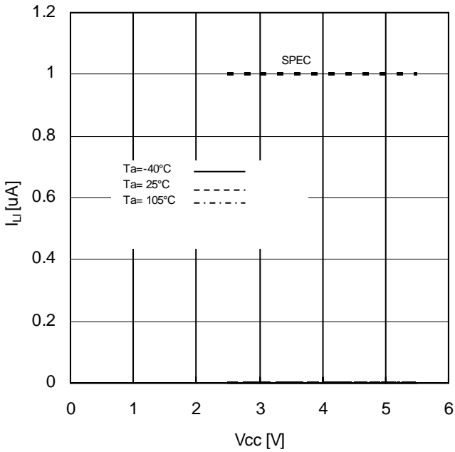
Figure 9. Input Leak Current vs Supply Voltage (CSB, SCK, SI, HOLDB, WPB)
