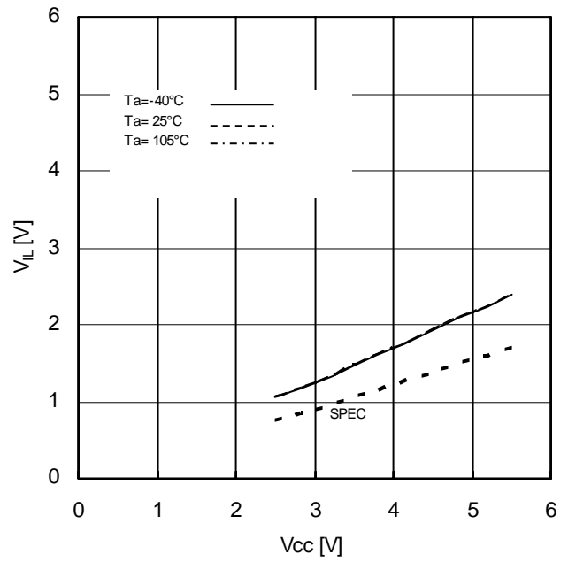
Figure 6. "L" Input Voltage vs Supply Voltage (CSB,SCK,SI,HOLDB,WPB)
