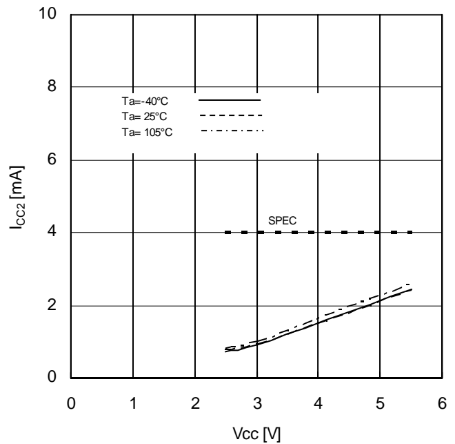
Figure 12 Current consumption at READ operation vs Supply Voltage
