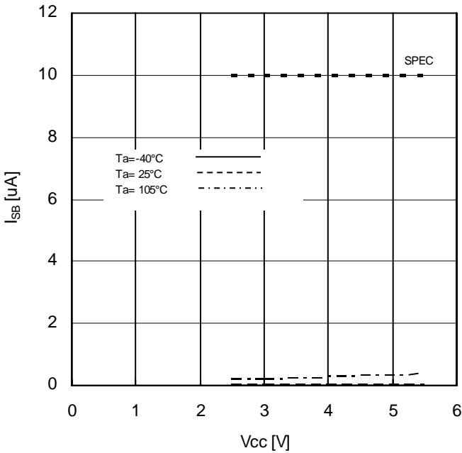
Figure 13. Current consumption at standby operation vs Supply Voltage
