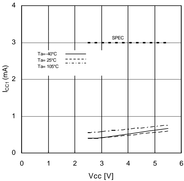
Figure 11. Current consumption at WRITE operation vs Supply Voltage
