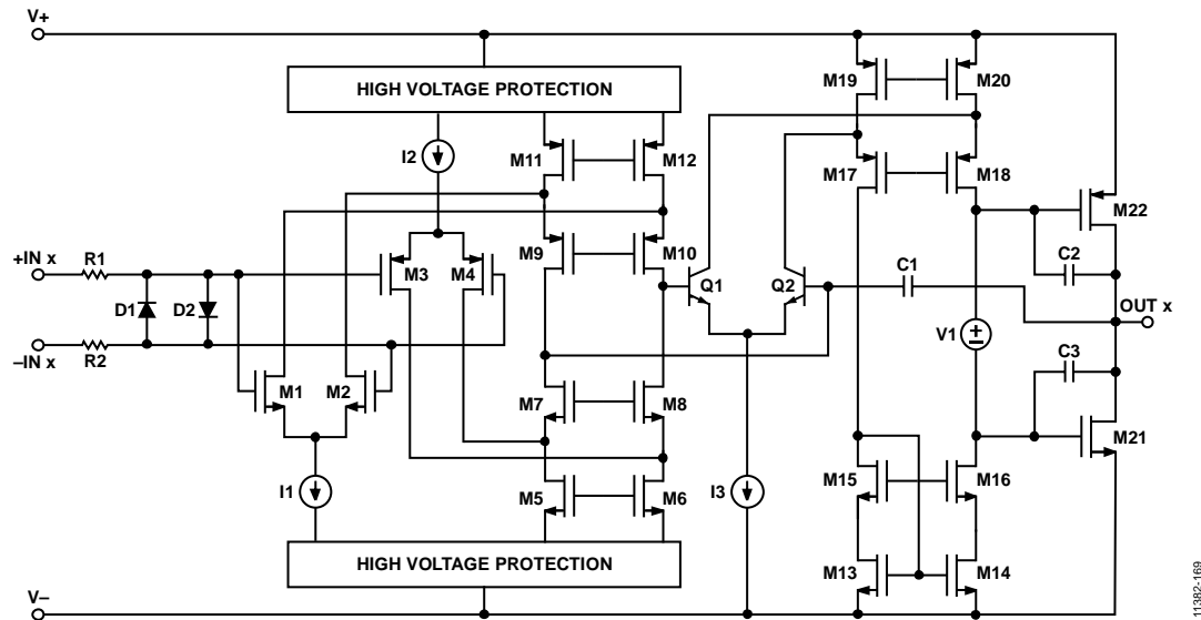
Figure 70. Simplified Schematic
