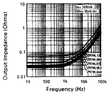
Output Impedance v Frequency
