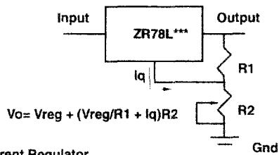
Current Regulator
