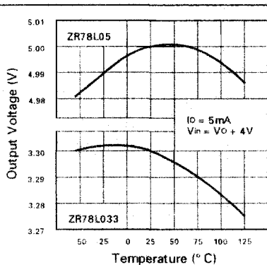
Output Voltage Temperature Coefficient
