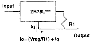
Current Regulator
