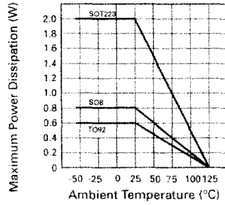
Power dissipation Derating
