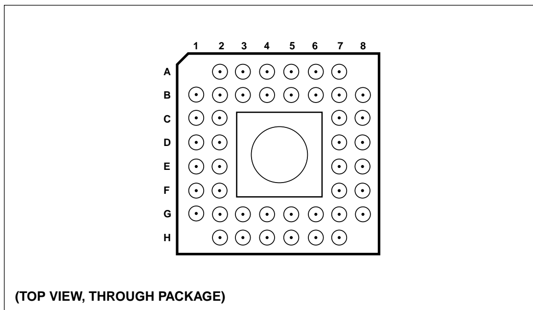
Figure 44. Drawing X2 – 44 Pin CPGA (Package Type X)
