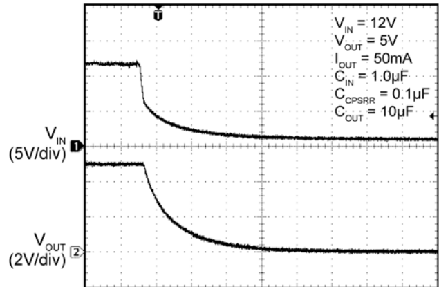
Hot Un-Plug
