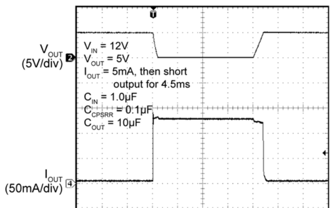
Current Limit
