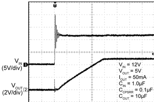
Hot Plug
