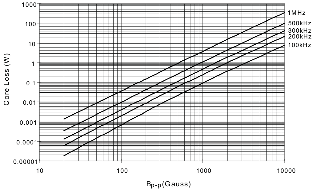
Core Loss vs B_{p-p}
