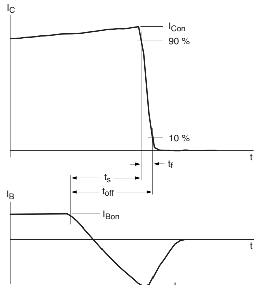
Fig 11. Switching times waveforms for inductive load
